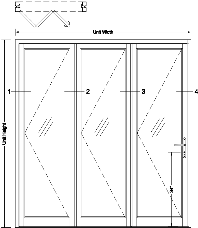
Bi-Fold Door (3 door)
