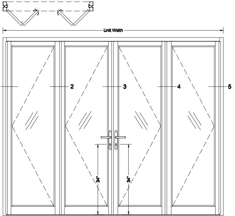
Bi-Fold Door (4 door both side open only)
